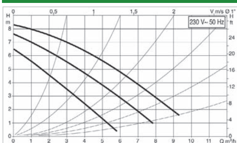
A 80/180 XM - B 80/250.40 M - D80/250.40 M
